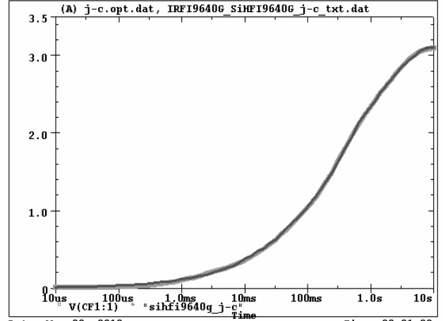
SiHFI9640G Filter j-c Temperature: 27.0
