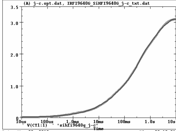
SiHFI9640G Tank j-c Temperature: 27.0
